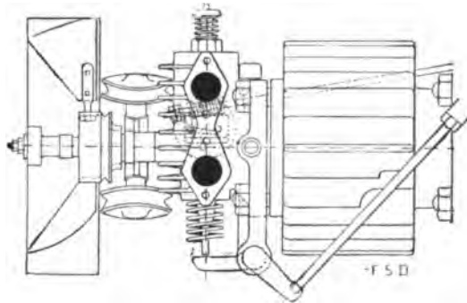
FIG. 299.—Detail Cylinder Head of the Simms Cycle Motor, showing fan wheel, cooling ribs, and peculiar arrangement for opening the exhaust. Similar fan wheels are used on several types of light vehicle motor.
